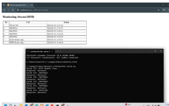
Fig 2. Monitoring RFID
